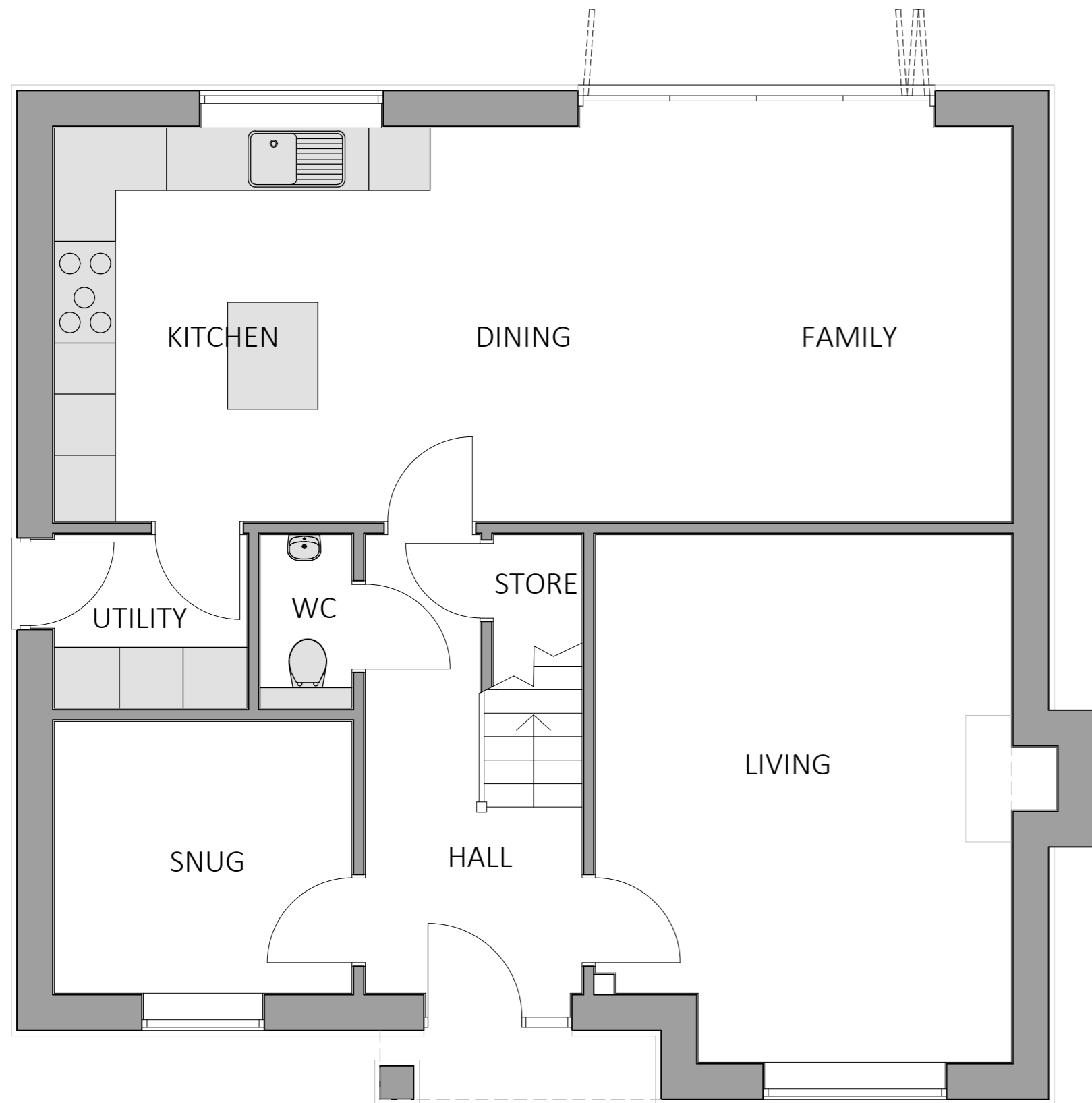
GROUND FLOOR - Plot 20
