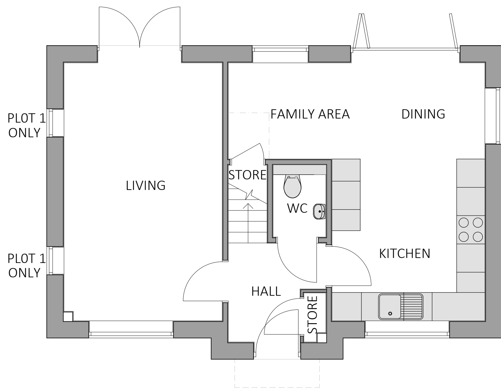
GROUND FLOOR - Plot 1,2 & 3
