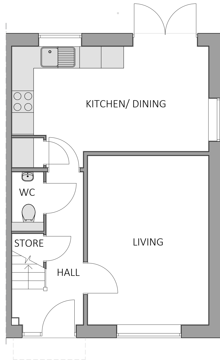
GROUND FLOOR - Plot 9 and 11 (Plot 8 and 10 handed)
