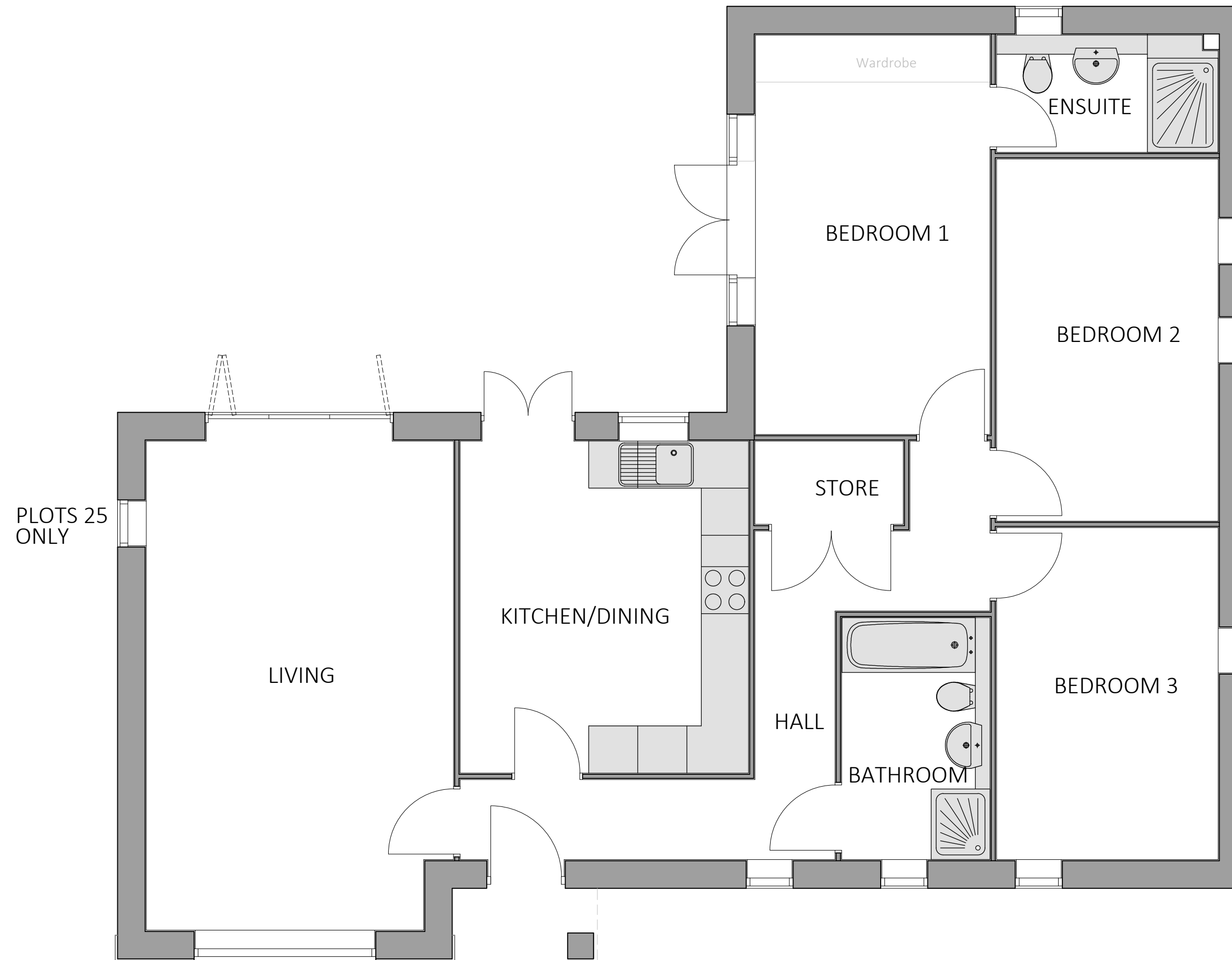
GROUND FLOOR - Plots 22 & 25 (Plots 6 & 17 handed)
